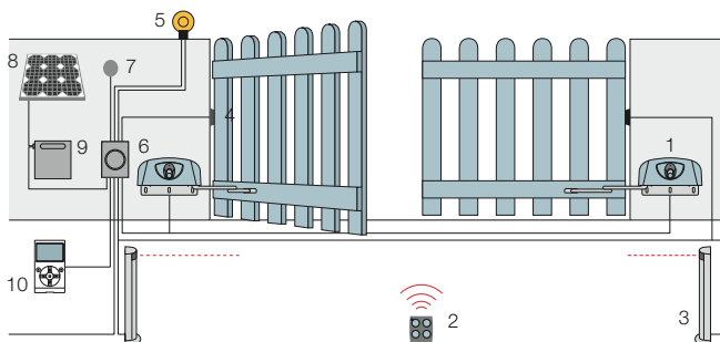
1. Hyppo 2. Transmitter 3. Photocells mounted on posts 4. Photocells 5. Flashing light 6. Control unit 7. Digital or key switches 8. SYP* solar panel 9. PSY24* battery box 10. O-View* multifunction display. *Optional connection to Solemyo and Opera systems.
